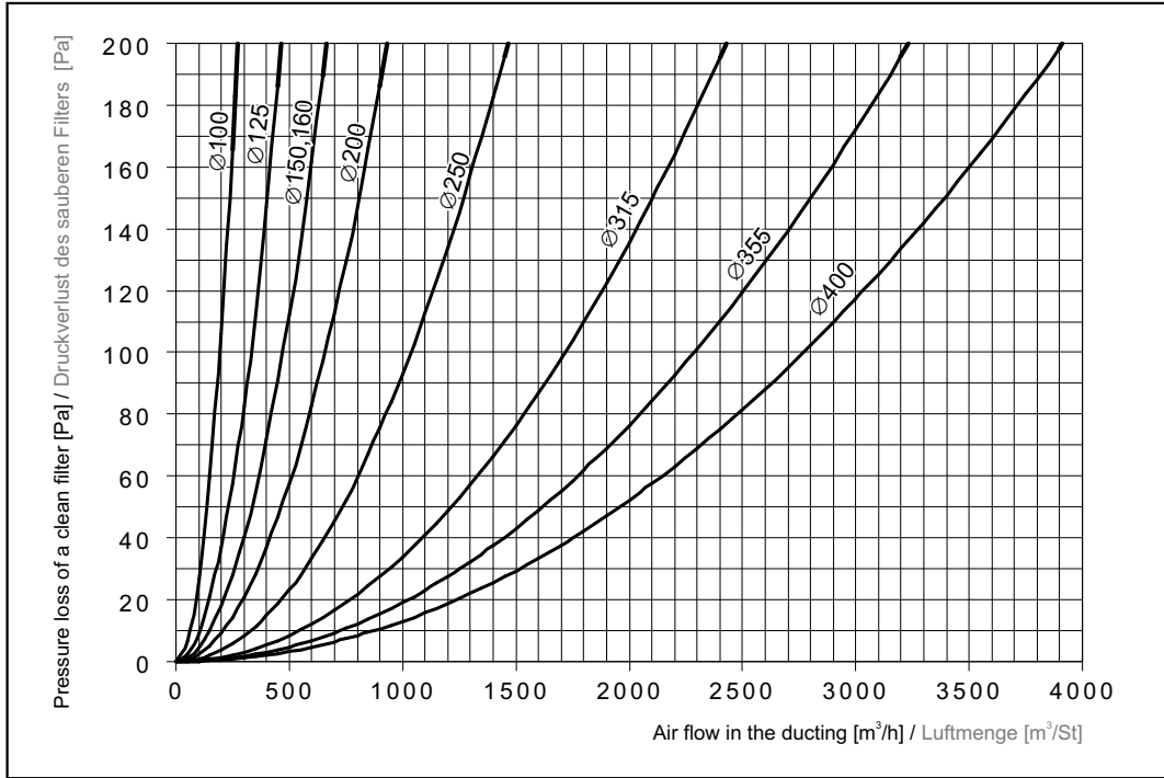
Pressure loss curves, filtration class G3
