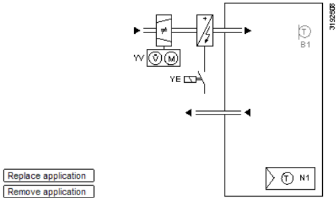
TBZB01 DU3 HQ - Single-duct with electric heater
