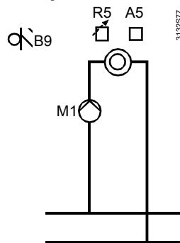
Weather-compensated pump heating circuit
