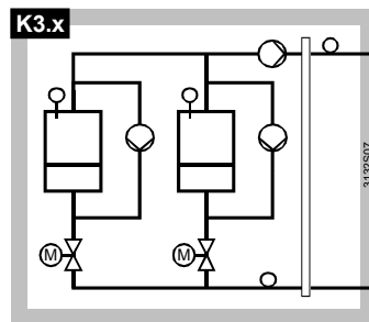
Multiboiler plant with: - 1 main pump in the common boiler flow - 1 bypass pump of each boiler - 1 shutoff valve in the return of each boiler
