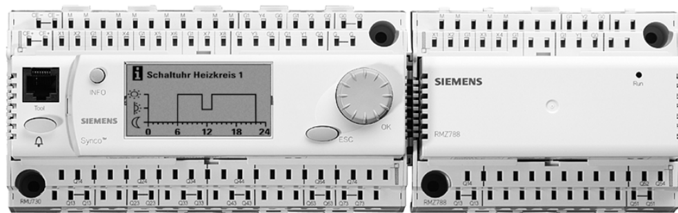
Universal controller RMU730 with plug-in operator unit RMZ790 and attached extension module RMZ788
