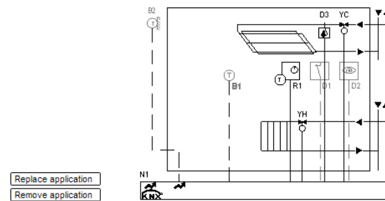
XCLC02 B24 HQ - Chilled ceiling
