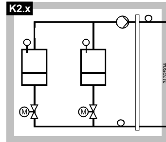
Multiboiler plant with: - 1 main pump in the common boiler flow - 1 shutoff valve in the return of each boiler
