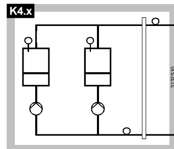
Multiboiler plant with: - 1 pump in the return of each boiler
