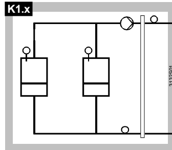
Multiboiler plant with: - 1 main pump in the common boiler flow
