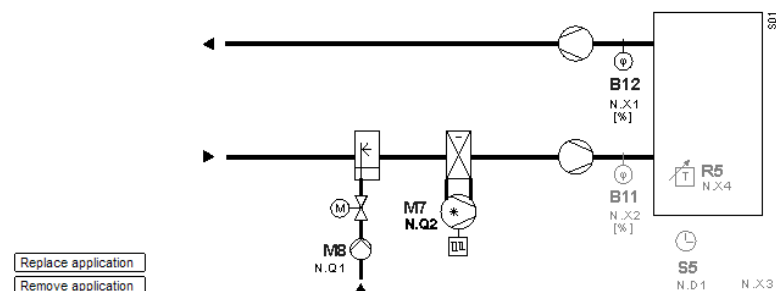
ADZA01 LU0 HQ - Ventilation Plant, Humidifying
