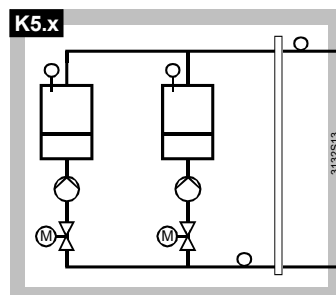
Multiboiler plant with: - 1 pump in the return of each boiler - 1 shutoff valve in the return of each boiler
