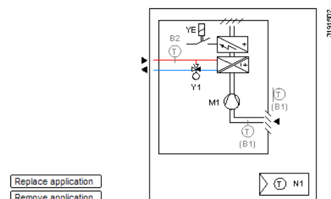
TAAB01 DG1 HQ - 2-pipe fan coil with electric heater
