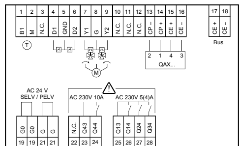
Connection terminals of RXL22.1
