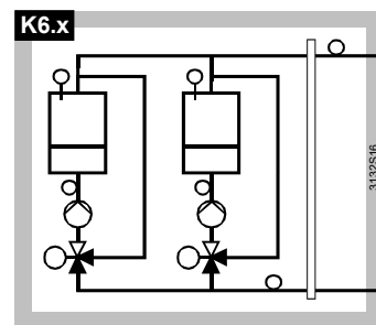
Multiboiler plant with: - 1 pump in the return of each boiler - Maintained return temperature of each boiler with mixing valve (modulating or 3-position)
