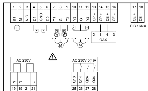
Connection terminals of RXB21.1
