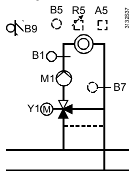
Weather-compensated heating circuit control
