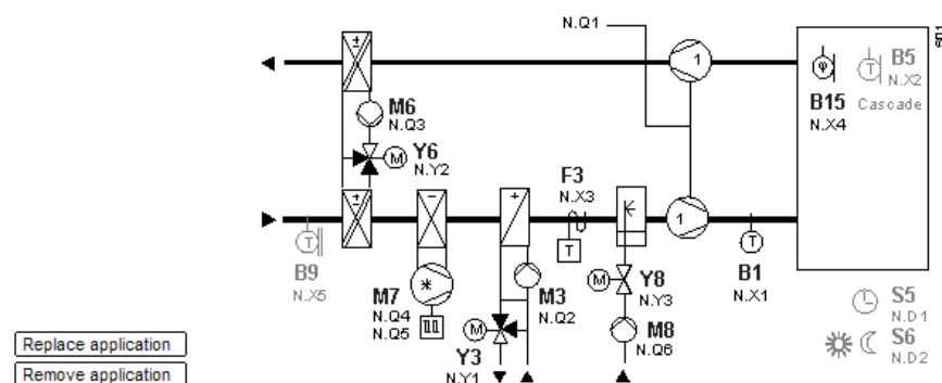
AEFL01 LU3 HQ - Partial Air Conditioning Plant, Heating / Cooling / Humidifying
