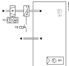
TBZB01 DG4 HQ - Single-duct with electric heater
