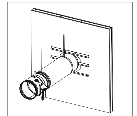
Close installation with L profiles 30x30x3mm. Additionally fix profiles to duct with self-tapping screws, and screw them to wall with 4,5x50 screws.
