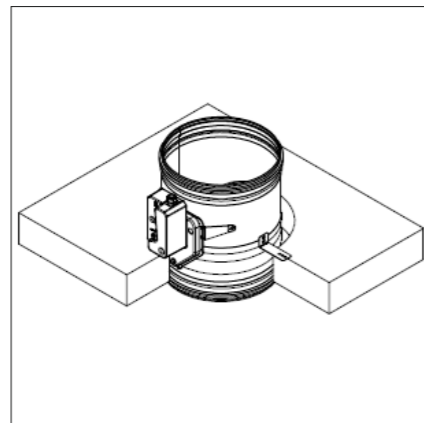
Fix the damper to the slab using screws
