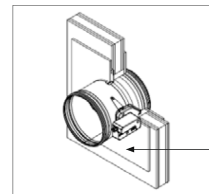
Cover the mineral wool with GKF gypsum boards (12,5 mm thick)
