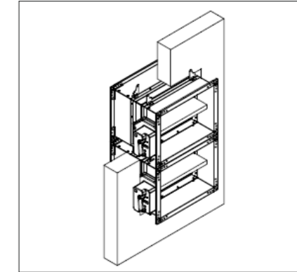
Fix the dampers to the wall using the screws and fill the space between the dampers and the wall with mortar
