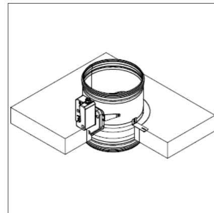
Fill the space between the damper and the slab with mortar
