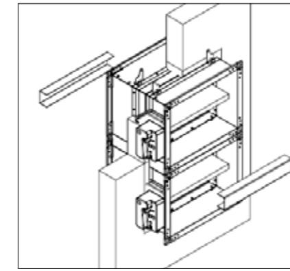
Place the installation kit to the dampers
