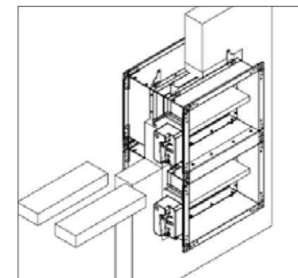
Fill the space between the dampers with mineral wool (100 kg/m 3 of density)
