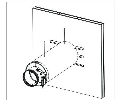
Additionally place steel protection on place where insulation on damper ends.
