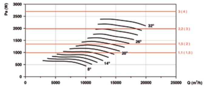
Absorbed power
