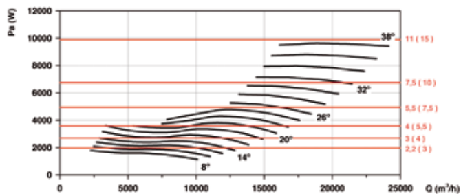
Absorbed power
