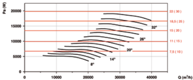
Absorbed power
