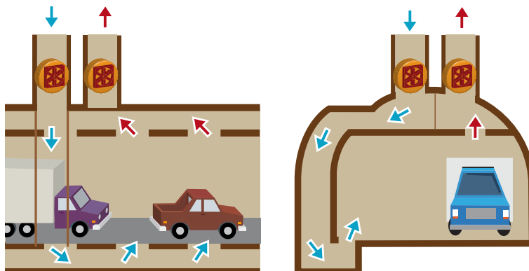
Transverse Ventilation
