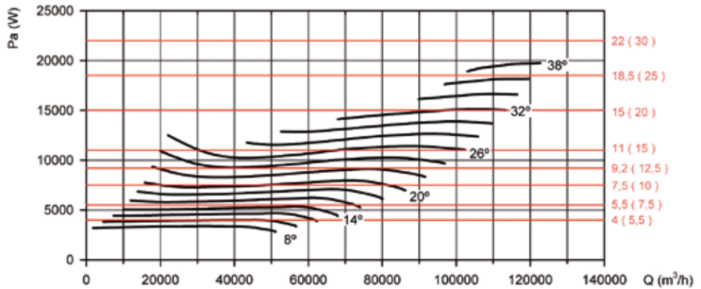
Absorbed power
